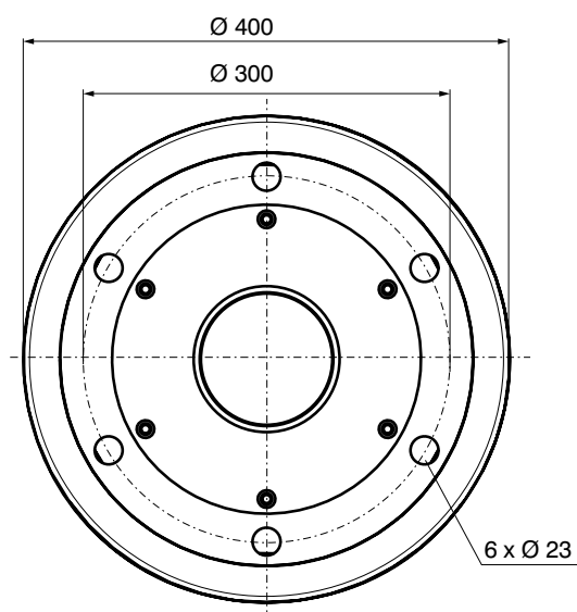
FLW 80-120 chuck with shaft end
